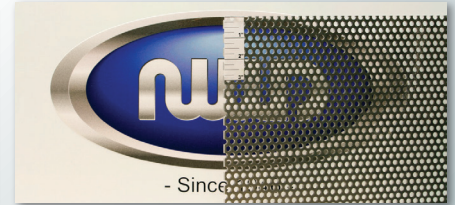
Perforated Panel - Mill Finish 40% Open Air, .25" Diameter Holes
